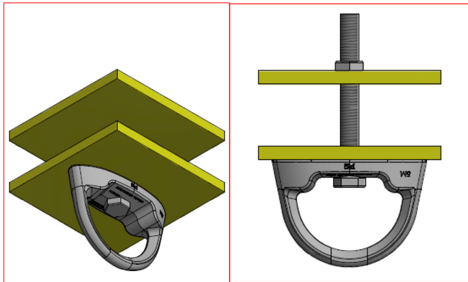
Figure 1 - Fixed Truss Anchor
