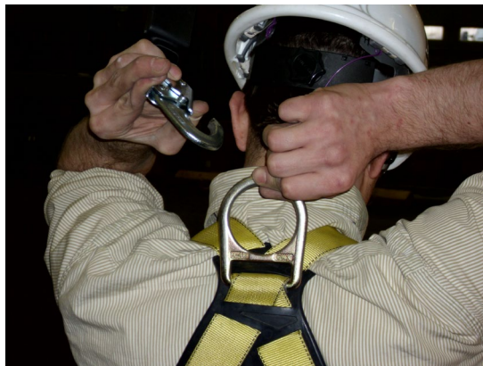
Figure 25 - Connect Snaphook to Harness
