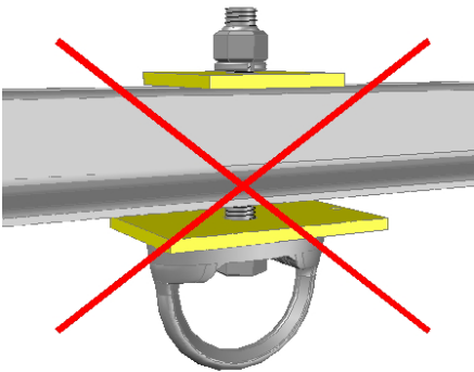
Figure 15 - Not Enough Torque
