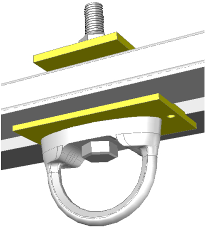
Figure 11 - Good Anchor Placement
