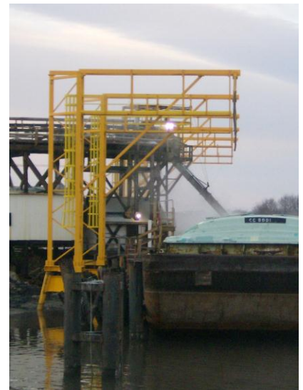
A rigid L gallows system used to load and unload ships safely
