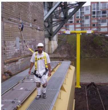
Walking safely across a rail car with the aid of a lifeline and a T Gallows system
